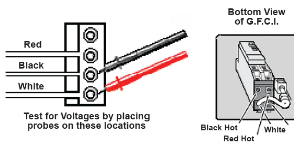
Figure 2. Proper Voltage Readings Across Terminals on House Breaker Box, Swim Spa and Exercise Pool System Box and GFCI
