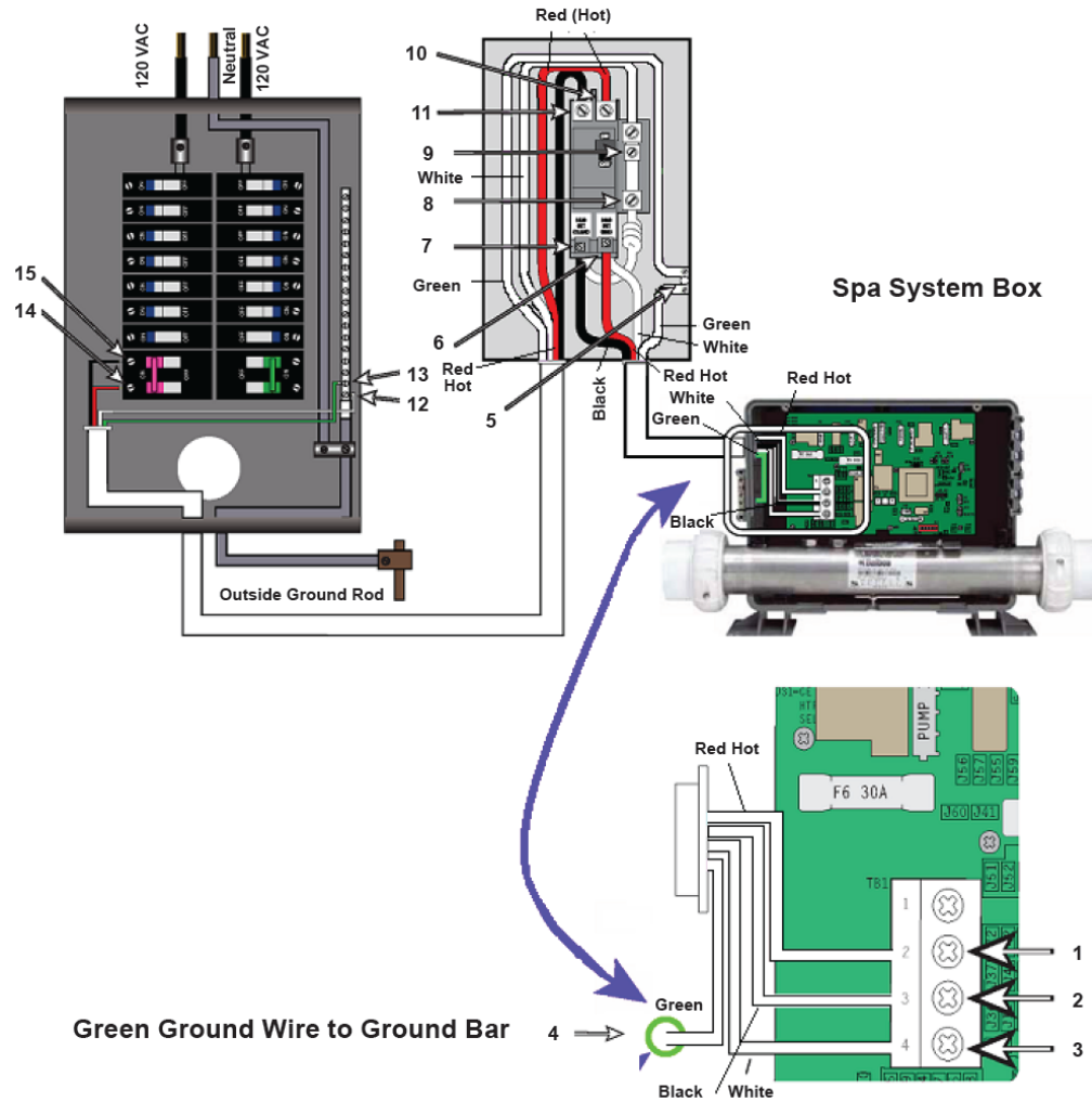
Figure 1. GFCI Wiring Schematic for 60 Hz Systems
